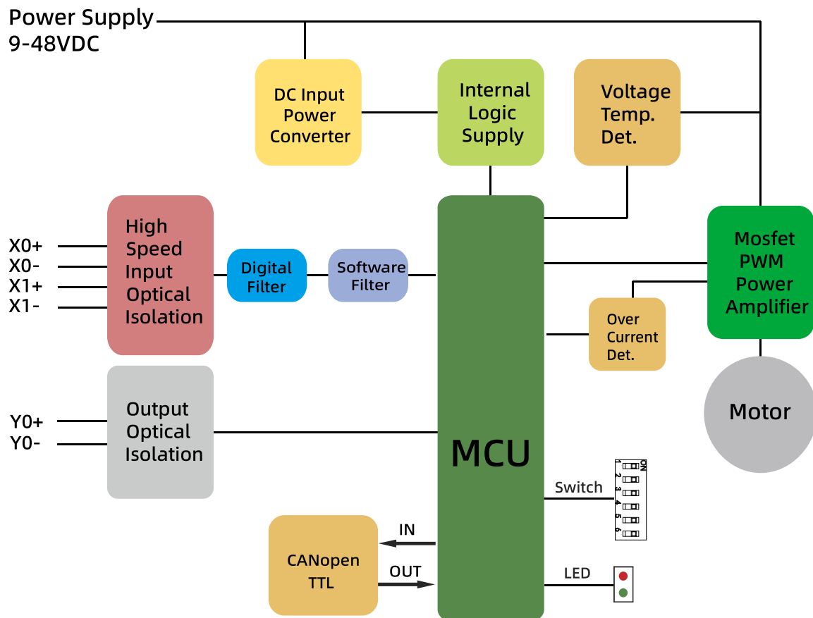
IG42EC Block Diagram
